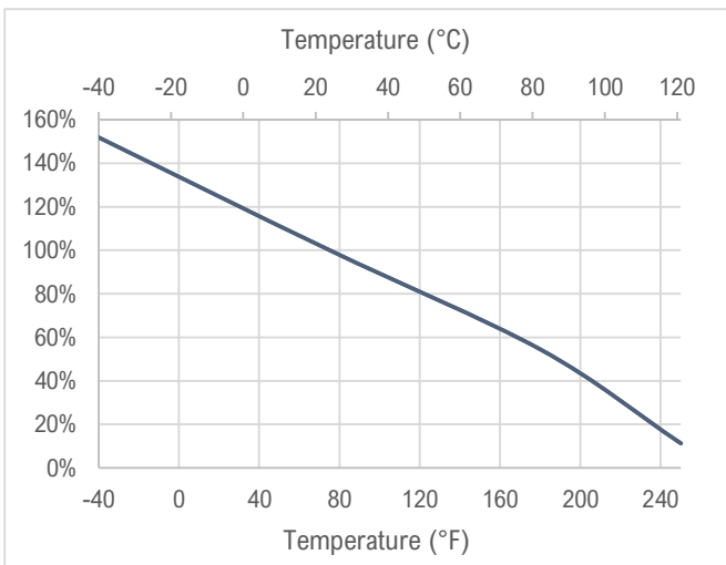
Strength Retention vs Temperature (ASTM D1002 on AI 6061)
