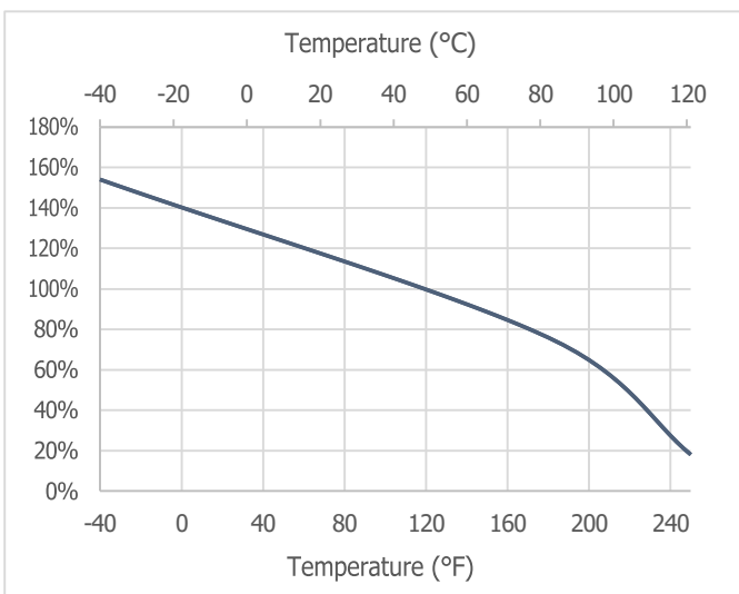
Strength Retention vs Temperature (ASTM D1002 on Al 6061)
