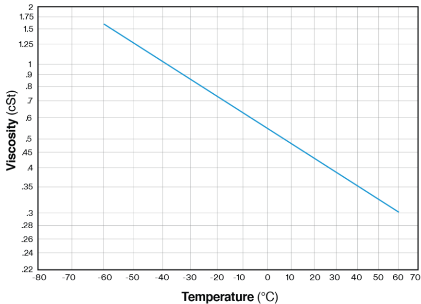
3M™ Fluorinert™ Electronic Liquid FC-3284 Viscosity vs. Temperature
