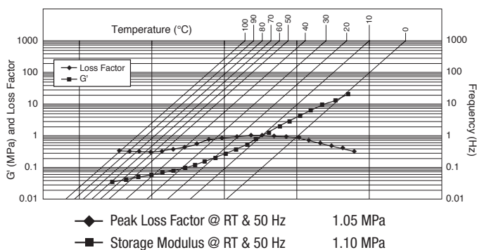
3M™ Ultra-Pure Viscoelastic Damping Polymer 242NR02 Nomograph
