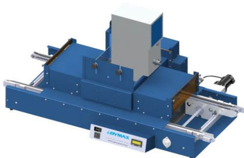
One center-mounted Fusion F300 for 6" wide exposure
